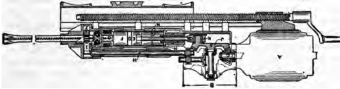
Fig. 41. Section Showing Details of Pneumelectric Rock Drill.
